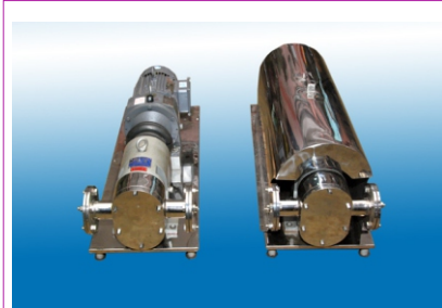
Lobe Pump With Base Frame & Cover
