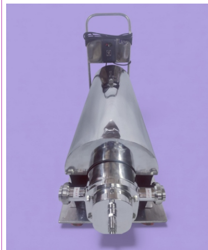
Jacketted Lobe Pump With Trolley & Cover
