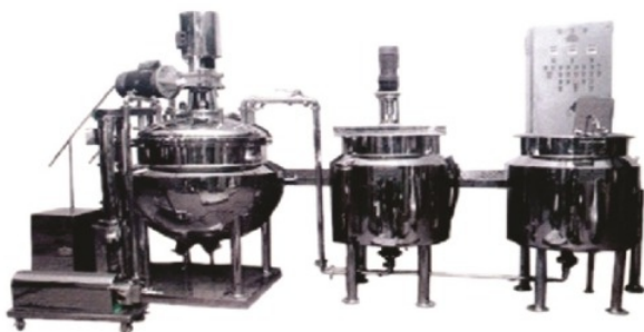
Ointment Cream Manufacturing Plant
