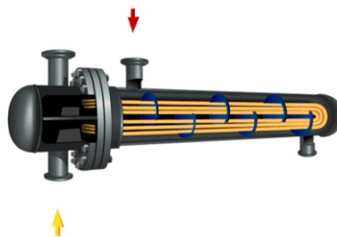
U-Tube-Heat-Exchanger
